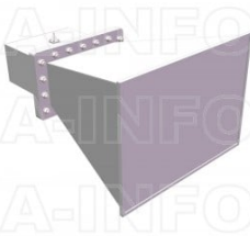
LB-975-10-C-SFSPO Standard Gain Horn Antenna 0.75-1.12GHz 10dB Gain SMA Female
